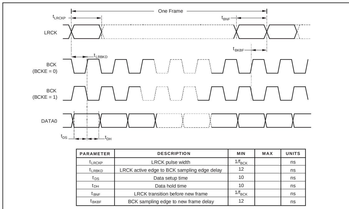
Figure 15. TDM Timing
