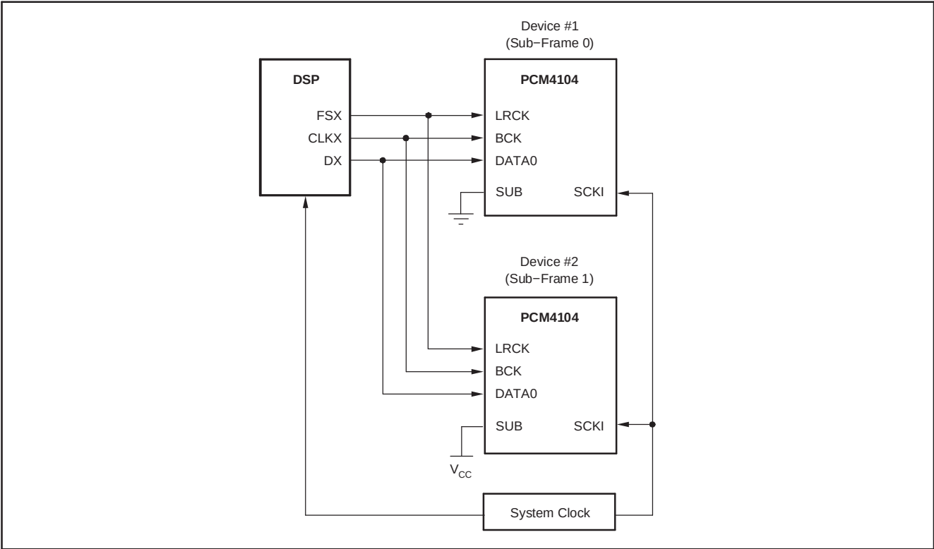
Figure 12. TDM Connection
